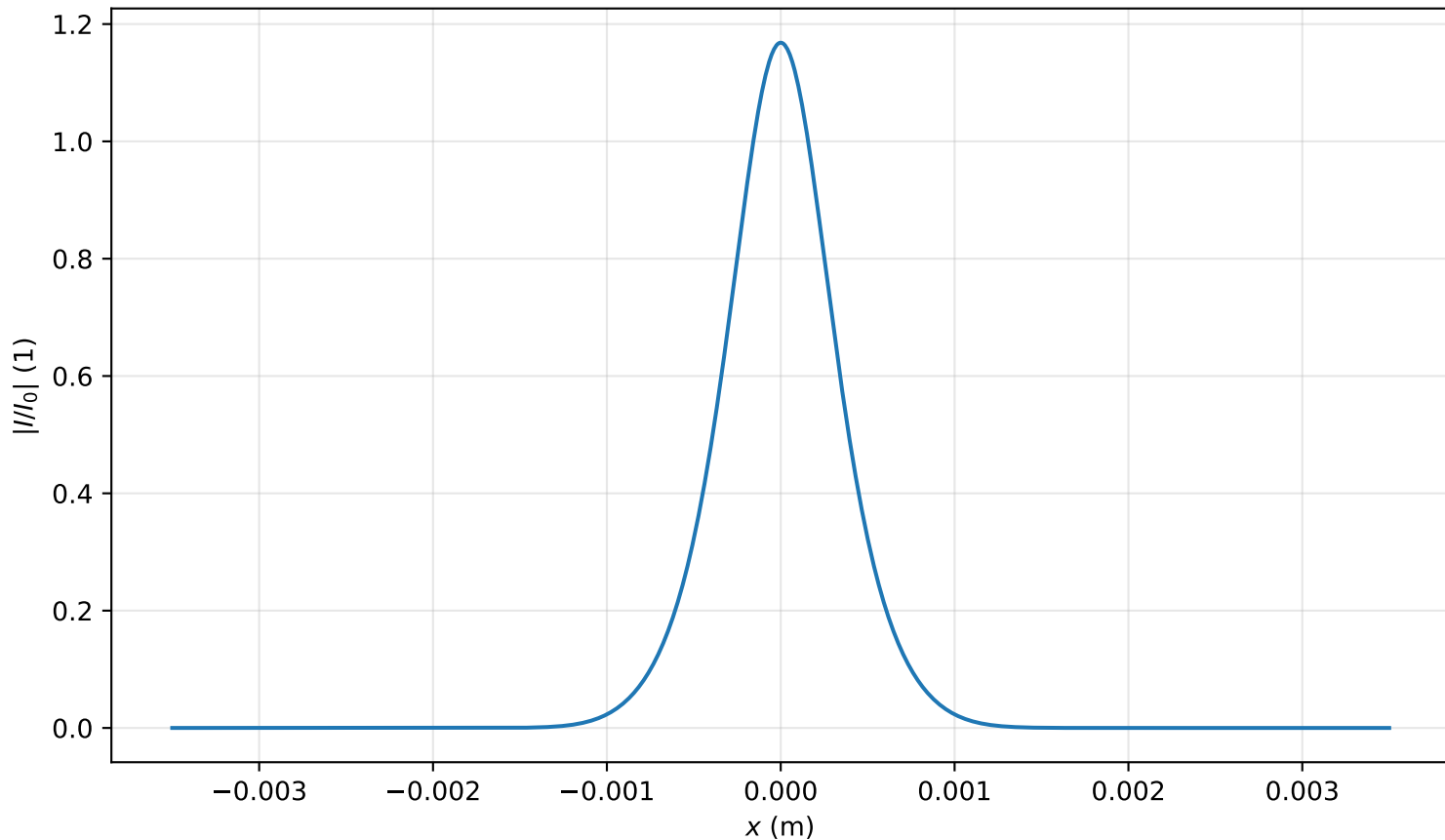
Intensity profile I(x, y = 0, z = 0.796m)/I_0 , P_{in}=0.7P_{cr} , artificial time
